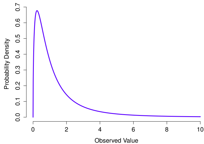
Figure 9.11: An F distribution with 3 and 5 degrees of freedom. Qualitatively speaking, it looks pretty similar to a chi-square distribution, but they’re not quite the same in general.
