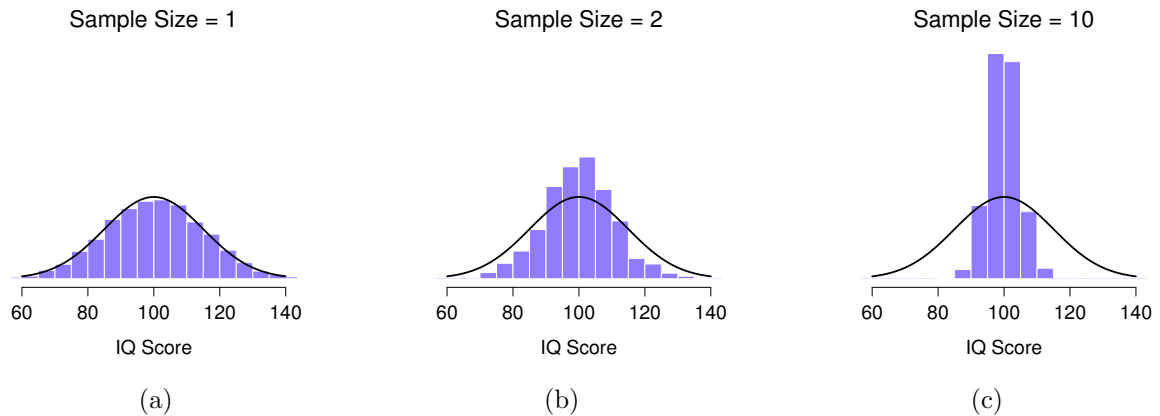
Figure 10.3: An illustration of the sampling distribution of the mean. In each panel, I generated 10,000 samples of IQ data, and calculated the mean IQ observed within each of these data sets. The histograms in these plots show the distribution of these means (i.e., the sampling distribution of the mean). Each individual IQ score was drawn from a normal distribution with mean 100 and standard deviation 15, which is shown as the solid black line). In panel a, each data set contained only a single observation, so the mean of each sample is just one person’s IQ score. As a consequence, the sampling distribution of the mean is of course identical to the population distribution of IQ scores. However, when we raise the sample size to 2, the mean of any one sample tends to be closer to the population mean than a one person’s IQ score, and so the histogram (i.e., the sampling distribution) is a bit narrower than the population distribution. By the time we raise the sample size to 10 (panel c), we can see that the distribution of sample means tend to be fairly tightly clustered around the true population mean.
