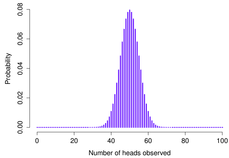
Figure 9.3: Two binomial distributions, involving a scenario in which I'm flipping a fair coin, so the underlying success probability is \theta = 1/2 . In panel (a), we assume I'm flipping the coin N = 20 times. In panel (b) we assume that the coin is flipped N = 100 times.
