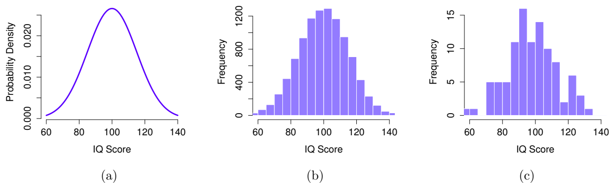
Figure 10.1: The population distribution of IQ scores (panel a) and two samples drawn randomly from it. In panel b we have a sample of 10,000 observations, and in panel c we have a sample of 100 observations
