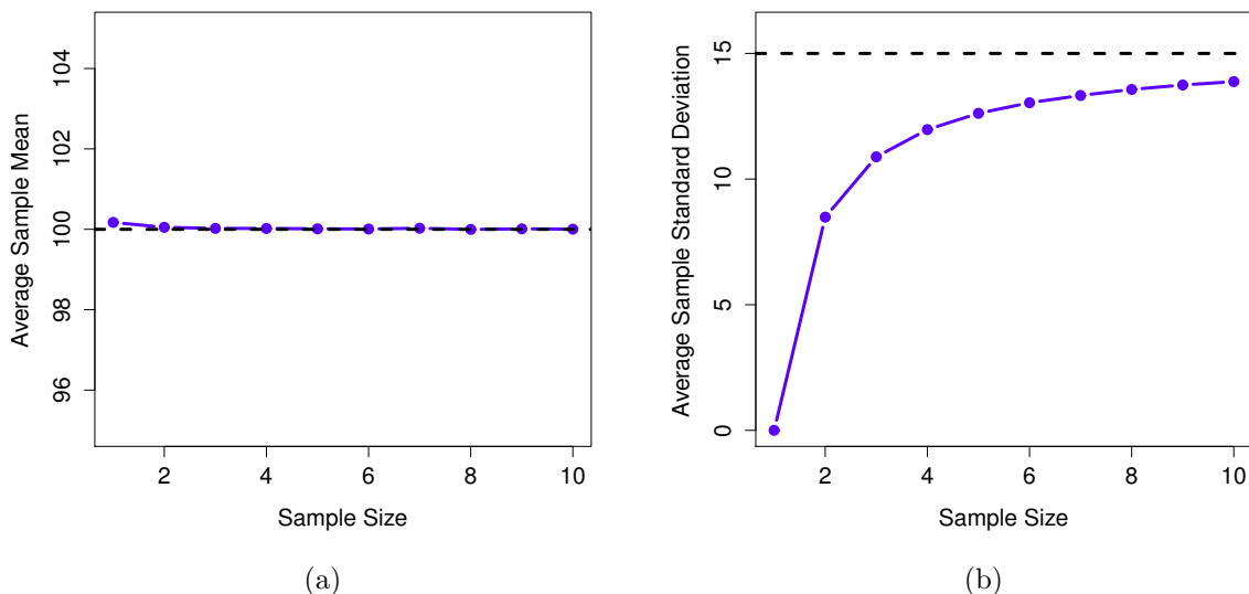
Figure 10.2: An illustration of the fact that the sample mean is an unbiased estimator of the population mean (panel a), but the sample standard deviation is a biased estimator of the population standard deviation (panel b). To generate the figure, I generated 10,000 simulated data sets with 1 observation each, 10,000 more with 2 observations, and so on up to a sample size of 10. Each data set consisted of fake IQ data: that is, the data were normally distributed with a true population mean of 100 and standard deviation 15. On average , the sample means turn out to be 100, regardless of sample size (panel a). However, the sample standard deviations turn out to be systematically too small (panel b), especially for small sample sizes.
