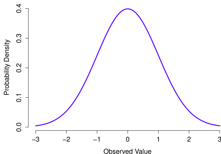
Figure 9.4: The normal distribution with mean \mu = 0 and standard deviation \sigma = 1 . The x -axis corresponds to the value of some variable, and the y -axis tells us something about how likely we are to observe that value. However, notice that the y -axis is labelled “Probability Density” and not “Probability”. There is a subtle and somewhat frustrating characteristic of continuous distributions that makes the y axis behave a bit oddly: the height of the curve here isn’t actually the probability of observing a particular x value. On the other hand, it is true that the heights of the curve tells you which x values are more likely (the higher ones!). (see Section 9.4.1 for all the annoying details)
