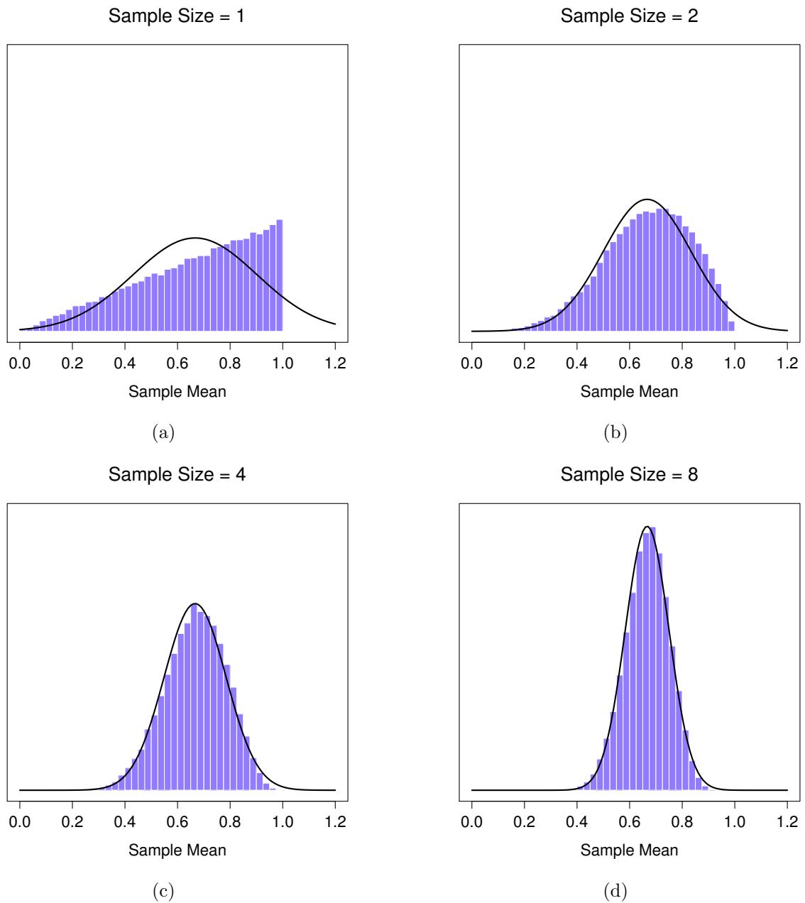
Figure 10.4: A demonstration of the central limit theorem. In panel a, we have a non-normal population distribution; and panels b-d show the sampling distribution of the mean for samples of size 2,4 and 8, for data drawn from the distribution in panel a. As you can see, even though the original population distribution is non-normal, the sampling distribution of the mean becomes pretty close to normal by the time you have a sample of even 4 observations.
