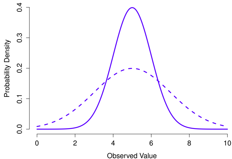
Figure 9.6: An illustration of what happens when you change the the standard deviation of a normal distribution. Both distributions plotted in this figure have a mean of \mu = 5 , but they have different standard deviations. The solid line plots a distribution with standard deviation \sigma = 1 , and the dashed line shows a distribution with standard deviation \sigma = 2 . As a consequence, both distributions are “centred” on the same spot, but the dashed line is wider than the solid one.
