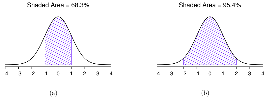
Figure 9.7: The area under the curve tells you the probability that an observation falls within a particular range. The solid lines plot normal distributions with mean \mu = 0 and standard deviation \sigma = 1 . The shaded areas illustrate “areas under the curve” for two important cases. In panel a, we can see that there is a 68.3% chance that an observation will fall within one standard deviation of the mean. In panel b, we see that there is a 95.4% chance that an observation will fall within two standard deviations of the mean.
