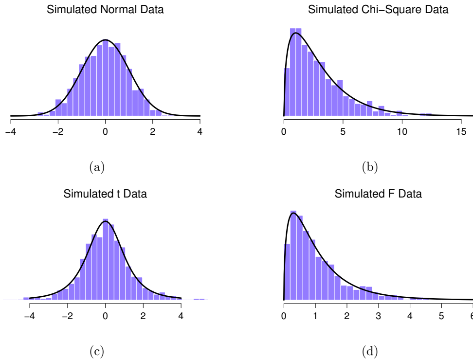
Figure 9.12: Data sampled from different distributions. See the main text for details.
