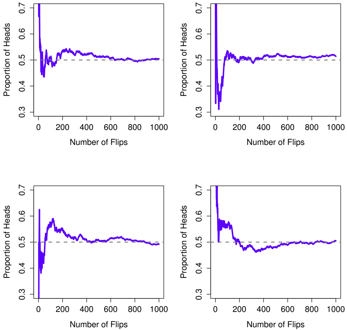
Figure 9.13: An illustration of how frequentist probability works. If you flip a fair coin over and over again, the proportion of heads that you've seen eventually settles down, and converges to the true probability of 0.5. Each panel shows four different simulated experiments: in each case, we pretend we flipped a coin 1000 times, and kept track of the proportion of flips that were heads as we went along. Although none of these sequences actually ended up with an exact value of .5, if we'd extended the experiment for an infinite number of coin flips they would have.
