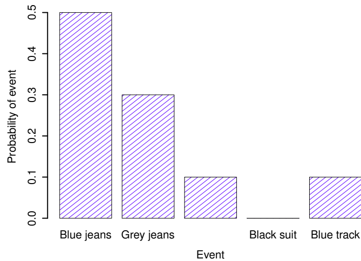
Figure 9.1: A visual depiction of the “pants” probability distribution. There are five “elementary events”, corresponding to the five pairs of pants that I own. Each event has some probability of occurring: this probability is a number between 0 to 1. The sum of these probabilities is 1.
