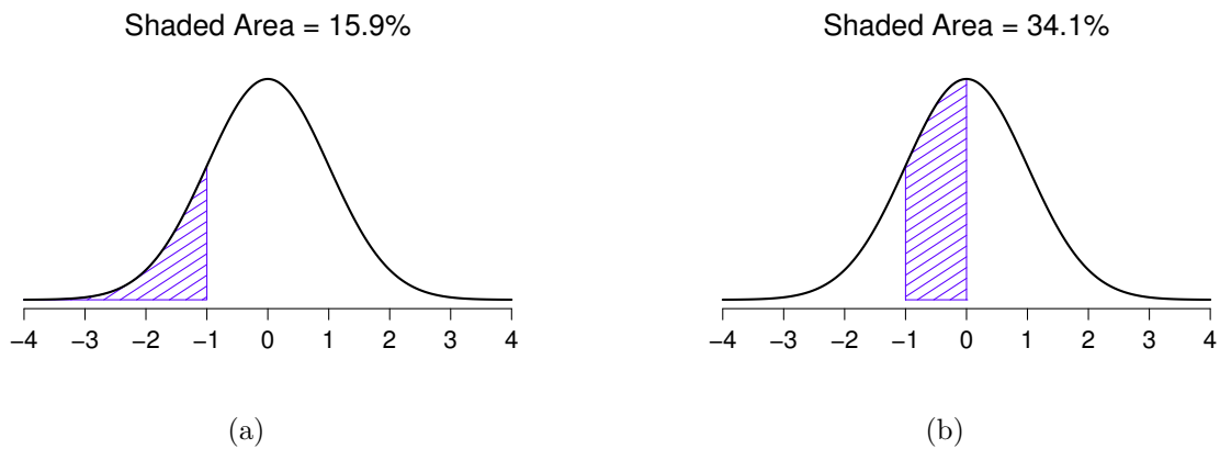
Figure 9.8: Two more examples of the “area under the curve idea”. There is a 15.9% chance that an observation is one standard deviation below the mean or smaller (panel a), and a 34.1% chance that the observation is greater than one standard deviation below the mean but still below the mean (panel b). Notice that if you add these two numbers together you get 15.9\% + 34.1\% = 50\% . For normally distributed data, there is a 50% chance that an observation falls below the mean. And of course that also implies that there is a 50% chance that it falls above the mean.
