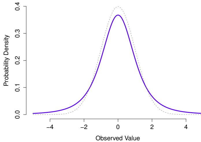
Figure 9.9: A t distribution with 3 degrees of freedom (solid line). It looks similar to a normal distribution, but it's not quite the same. For comparison purposes, I've plotted a standard normal distribution as the dashed line. Note that the "tails" of the t distribution are "heavier" (i.e., extend further outwards) than the tails of the normal distribution? That's the important difference between the two. .....
