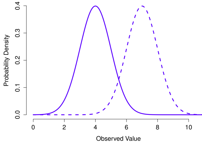
Figure 9.5: An illustration of what happens when you change the mean of a normal distribution. The solid line depicts a normal distribution with a mean of \mu = 4 . The dashed line shows a normal distribution with a mean of \mu = 7 . In both cases, the standard deviation is \sigma = 1 . Not surprisingly, the two distributions have the same shape, but the dashed line is shifted to the right.
