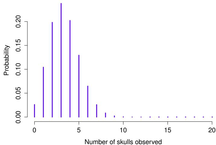
Figure 9.2: The binomial distribution with size parameter of N = 20 and an underlying success probability of \theta = 1/6 . Each vertical bar depicts the probability of one specific outcome (i.e., one possible value of X ). Because this is a probability distribution, each of the probabilities must be a number between 0 and 1, and the heights of the bars must sum to 1 as well.
