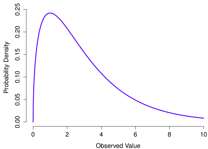
Figure 9.10: A \chi^2 distribution with 3 degrees of freedom. Notice that the observed values must always be greater than zero, and that the distribution is pretty skewed. These are the key features of a chi-square distribution. .....
