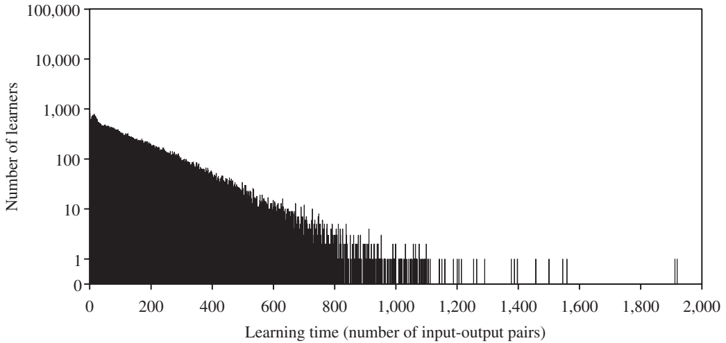
Figure 2 Histogram of convergence times of 100,000 Minimal GLA learners
