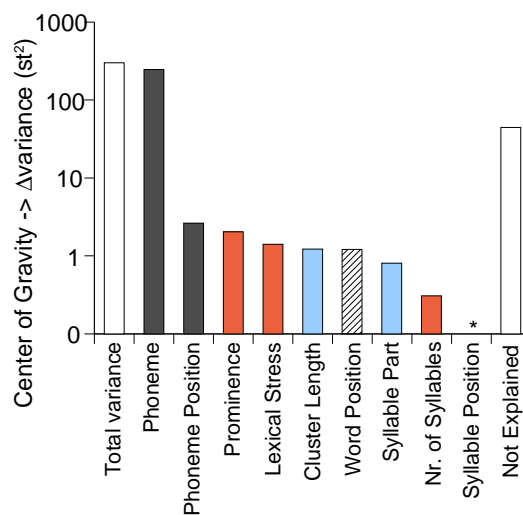
Figure 3. As Fig 2, but now for spectral Center of Gravity (in semitones). N=85,890 , maximal number of subsets: 38,795. All factors p<0.001 (F-test) except Syllable position (*, not significant). Not Explained variance: 14.9% of Total variance.
